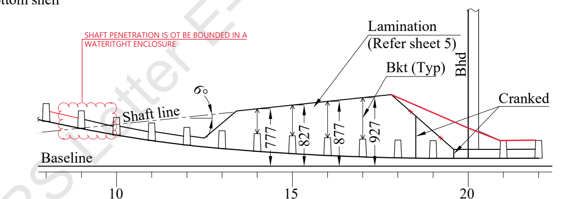
PROFILE IN WAY OFF ENGINE GIRDER (385MM OFF CL) (Height of Girder is indicative. Height to be adjusted to suite final shaft alignment at site)
