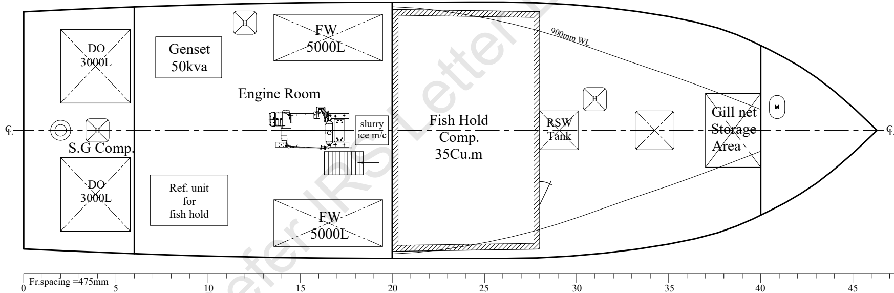
BELOW MAIN DECK
