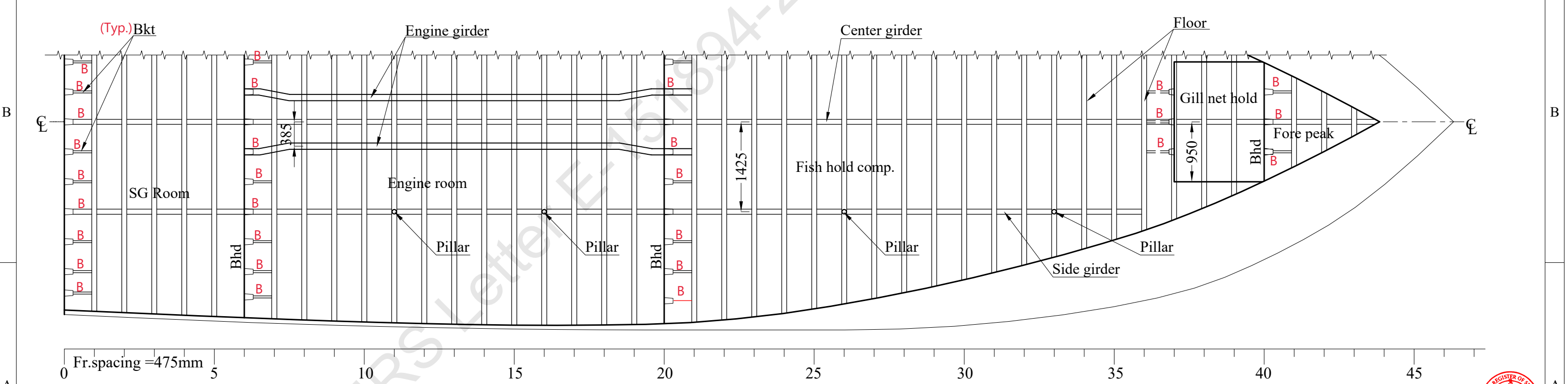
BOTTOM PLAN
