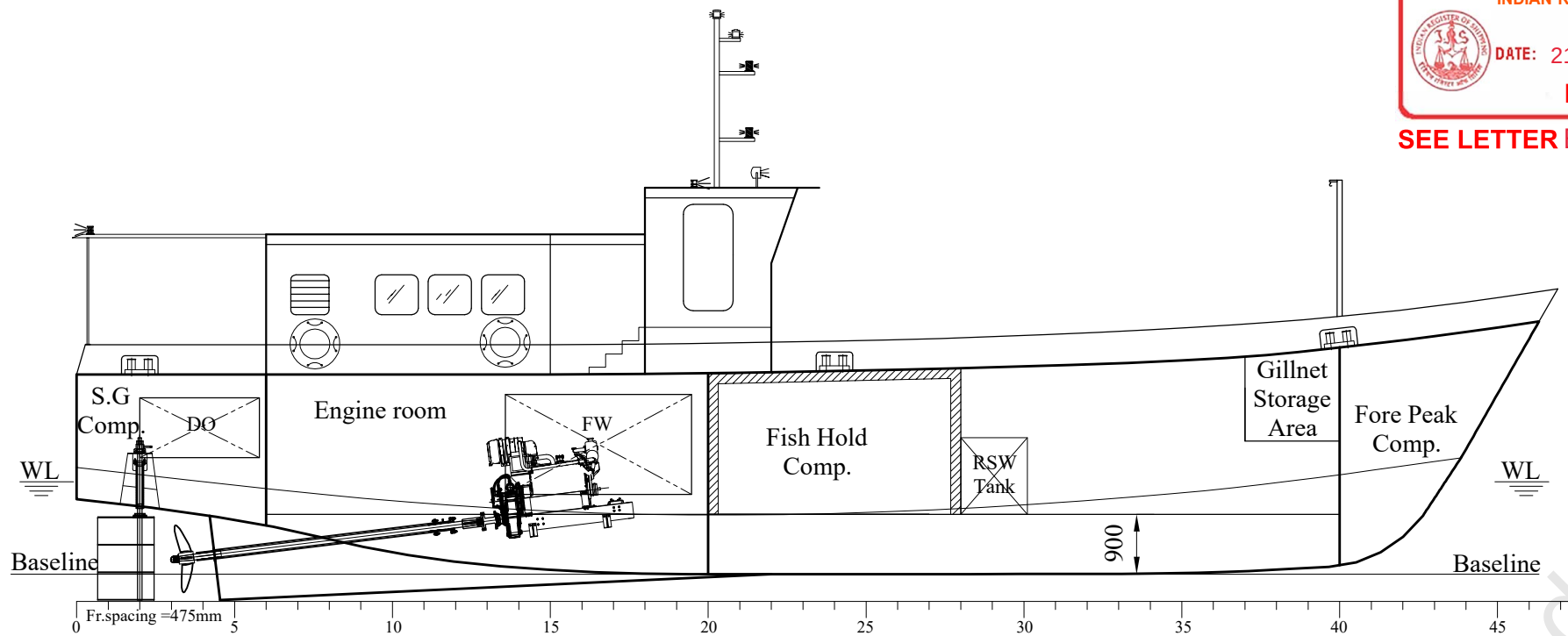
PROFILE
