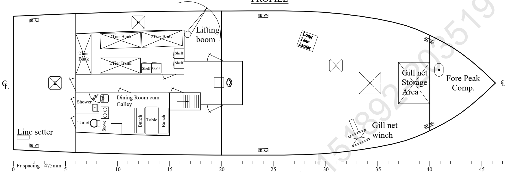
MAIN DECK
