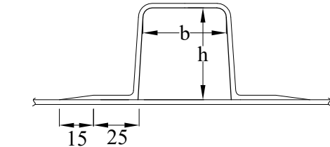
TYPICAL DECK BEAM/SIDE FRAME LAP
