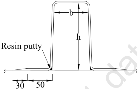
TYPICAL FLOOR/GIRDER LAP
