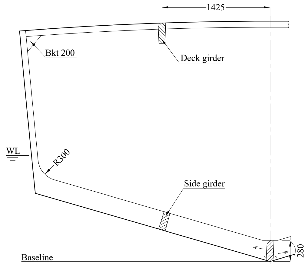
FR.22 (TYPICAL FRAME)
