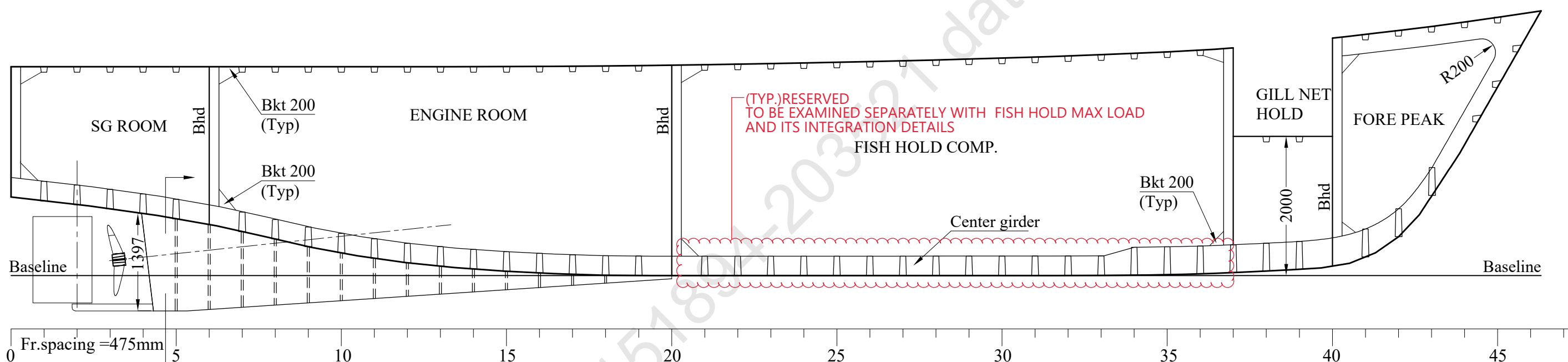
CENTERLINE PROFILE
